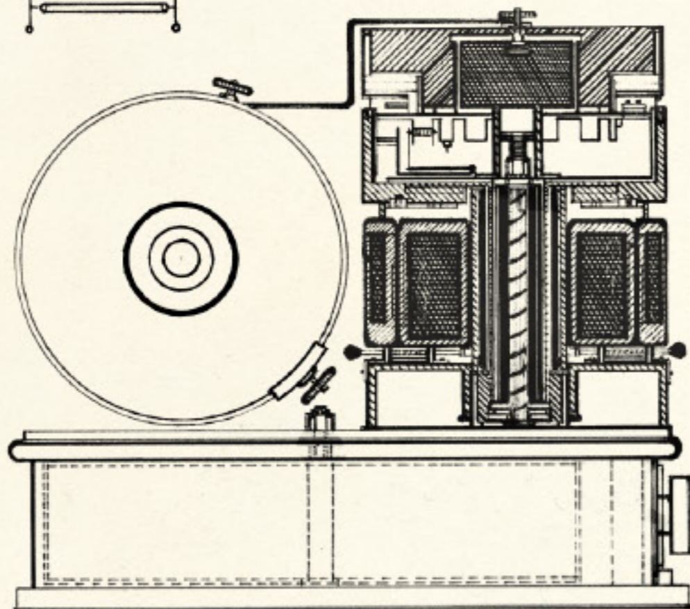
Fig. C1.3 section view electromechanical oscillator
